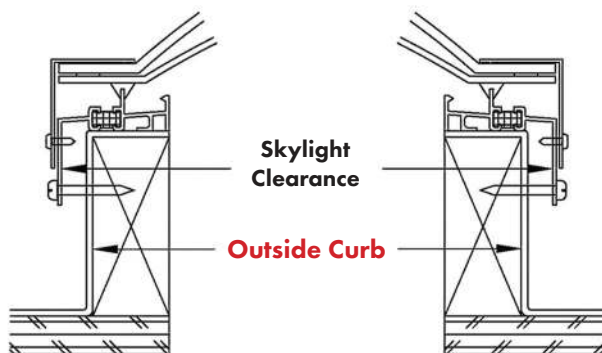
CURB-MOUNT SKYLIGHT
