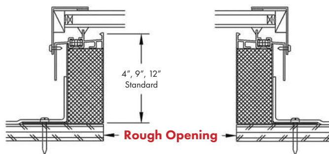
INSULATED CURB ("DECK-MOUNT") SKYLIGHT
